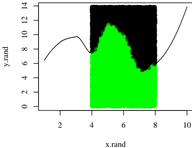
Integration from 4 to 8 = 33.25
