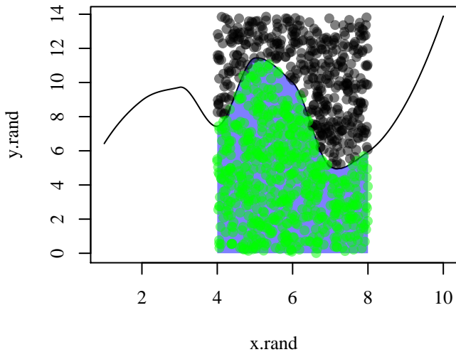
Integration from 4 to 8 = 32.92
