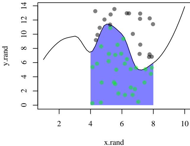
Integration from 4 to 8 = 32.92
