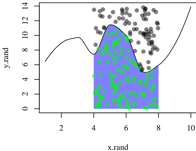
Integration from 4 to 8 = 33.25
